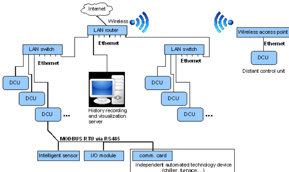
Figure 4: DCU networking.
