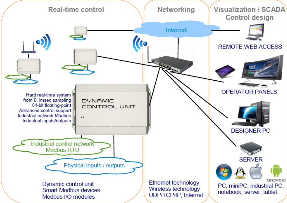
Figure 2: General structure of DCU Control System.
